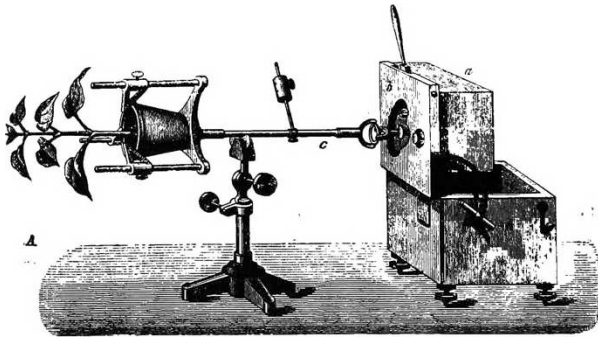
Fig. 4. Illustration showing the simple clinostat. Used under creative commons license. [9]
